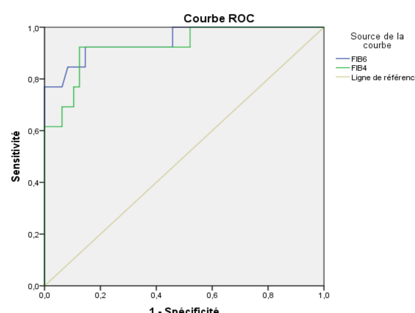
FIB-4
